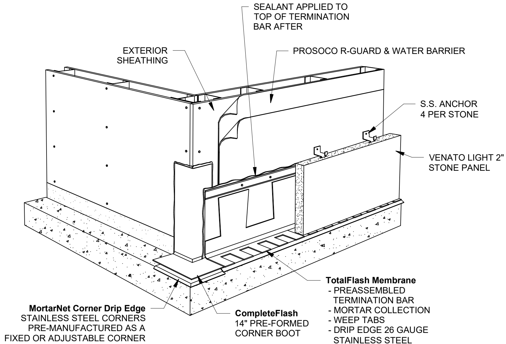
ASC ANCHORED STONE PANEL WITH TOTALFLASH - PERSPECTIVE
